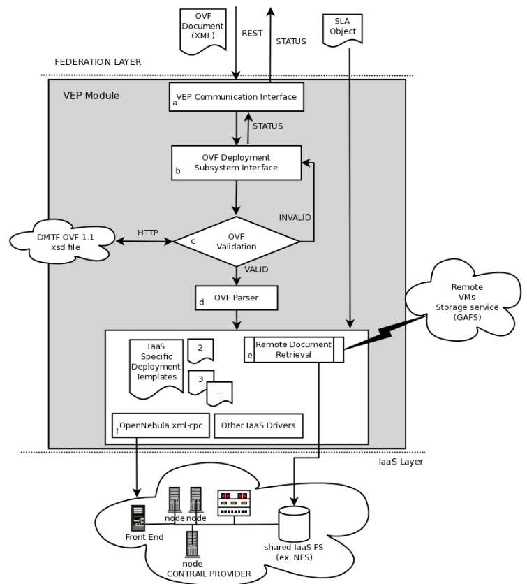
Fig. 3. OVF Centric VEP Deployment Taskflow
